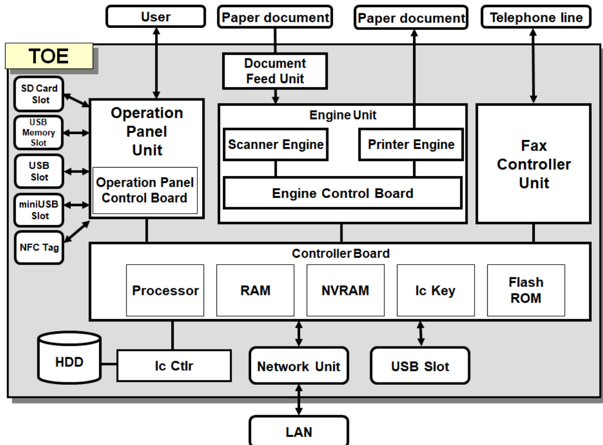
Figure 2 : Hardware Configuration of the TOE
